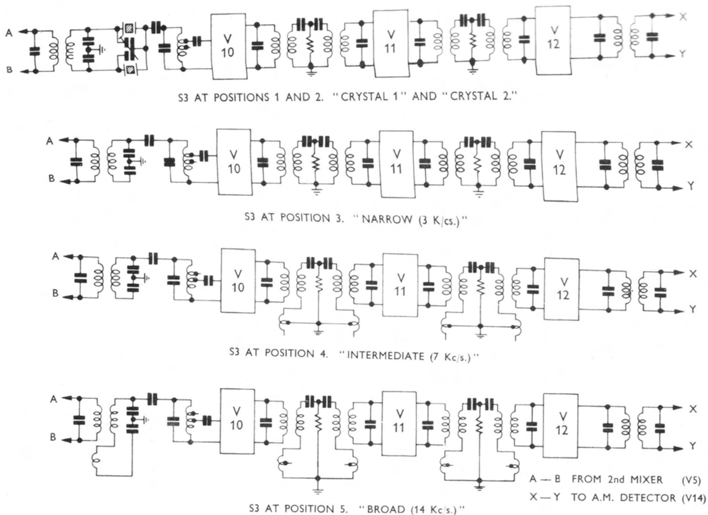
Fig. 4. Coupling arrangements at each position of Selectivity Switch
