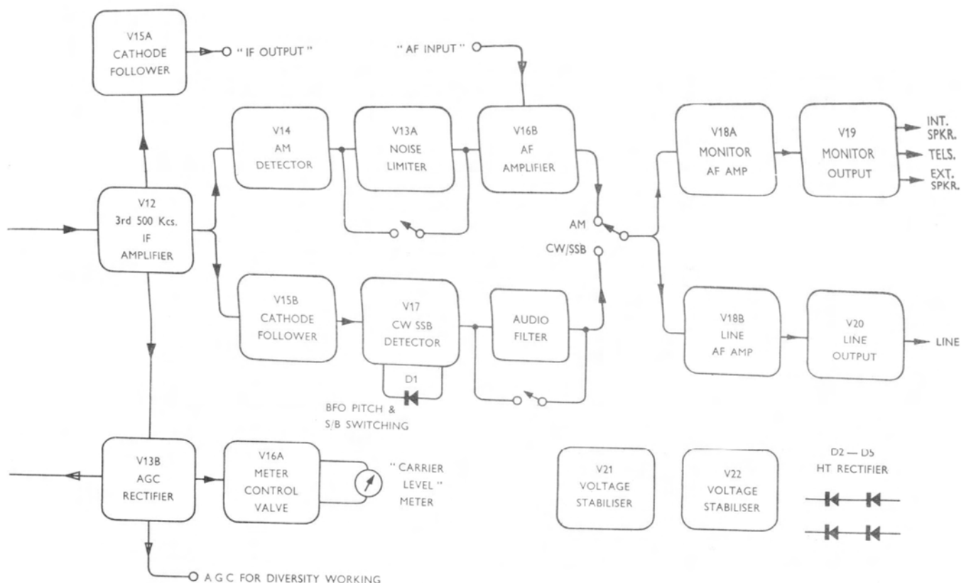
Fig 3. Block Schematic Diagram — Model 880/2.
